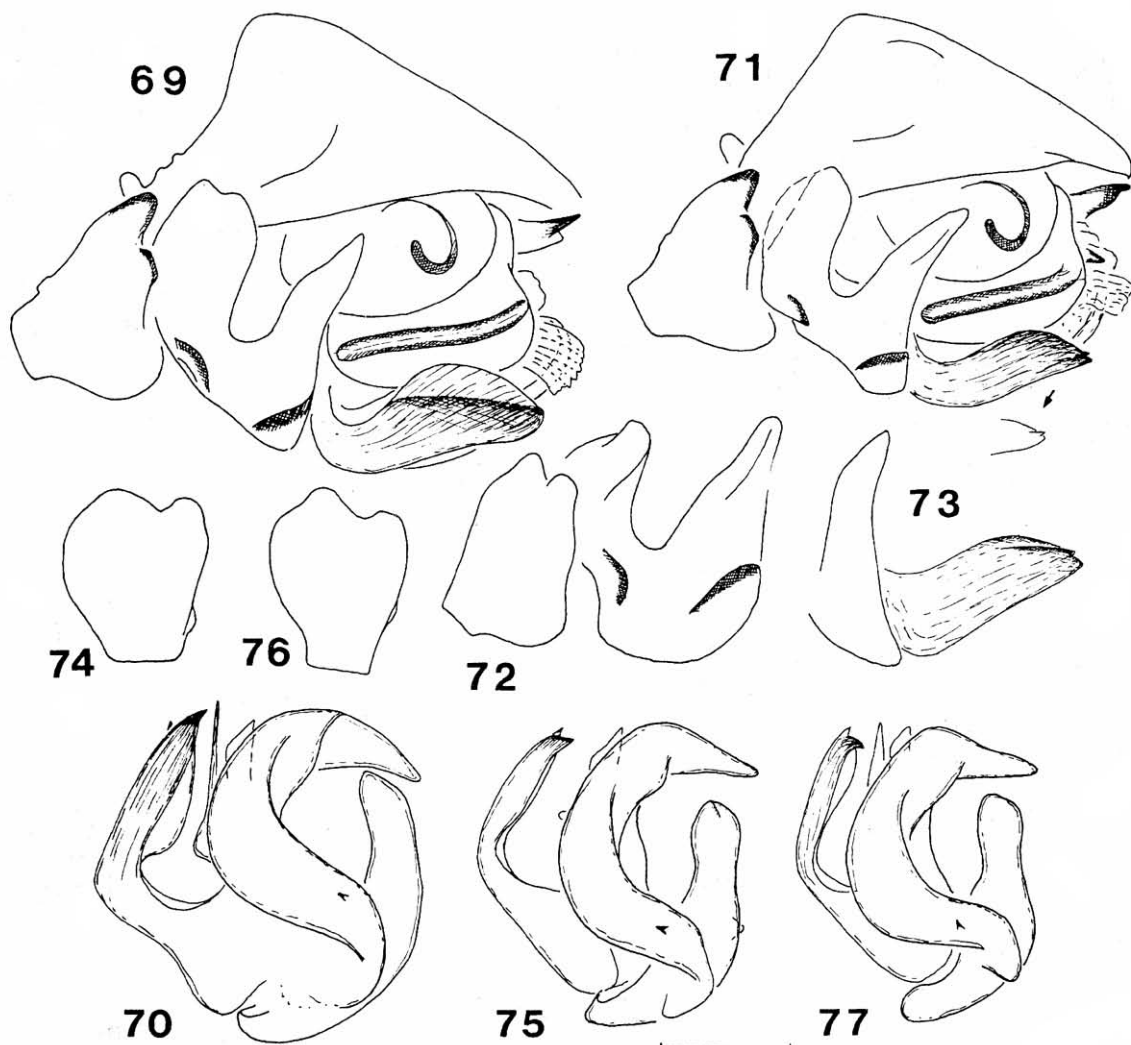
Figs 69–77. Details of palp structure of Agyneta resslī (Wunderlich, 1973) (69, 70, Austria, Gaming, paratype) & Agyneta mesasiatica sp.n. (71–77): 69, 71 — right palp, 72 — palpal tibia & paracymbium, 73 — lamella characteristica, 74, 76 — palpal tibia (dorsal view), 70, 75, 77 — embolic division (ventral view); 71–75 — Talysh Mts, Zuvand, holotype, 76, 77 — Baku.
