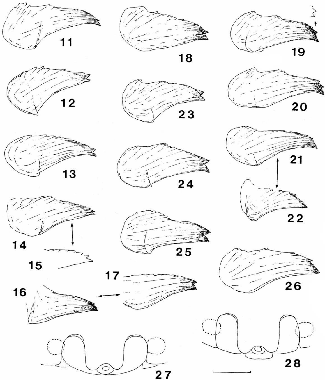
Figs 11–28. Lamella characteristic (11–26) and epigyne (27, 28) of Agymeta similis (Kulczyński, 1926): 11–15, 27 — Kamchatka, Geysers Valley, 16, 17, 28 — Yamal Peninsula, 18–22 — Polar Urals, 23 — Vorkuta, 24 — Shapkina River, 25 — Tobseда, 26 — Utsjoki Kevo Jesnalvaara (Finland).
