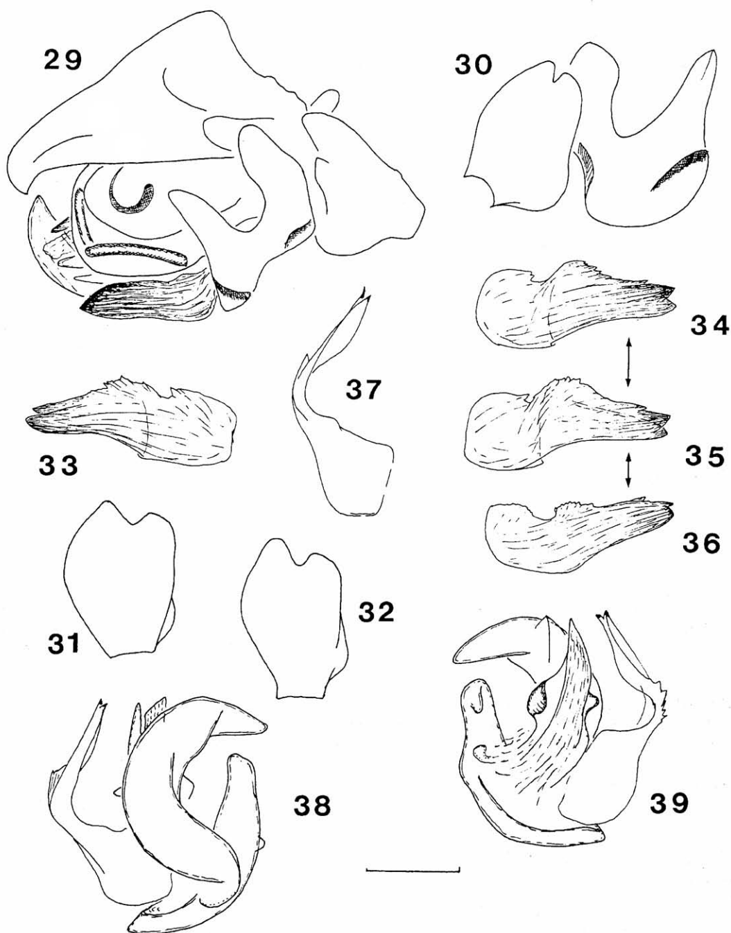
Figs 29–39. Details of palp structure of Agyreta insulana sp.n. (Iturup Island, holotype): 29 — left palp, 30 — palpal tibia & paracymbium, 31, 32 — palpal tibia, 33–37 — lamella characteristica (37 — ventral view!), 38, 39 — embolus division (ventral and dorsal views, respectively).
